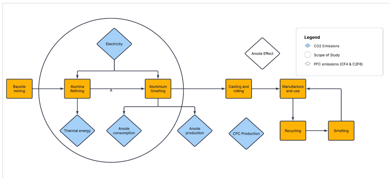
Figure 1 High-level overview of the aluminum sector describing processes and sources of GHG emissions. The scope of this study, primary aluminum production emissions, is enclosed by a circle.
