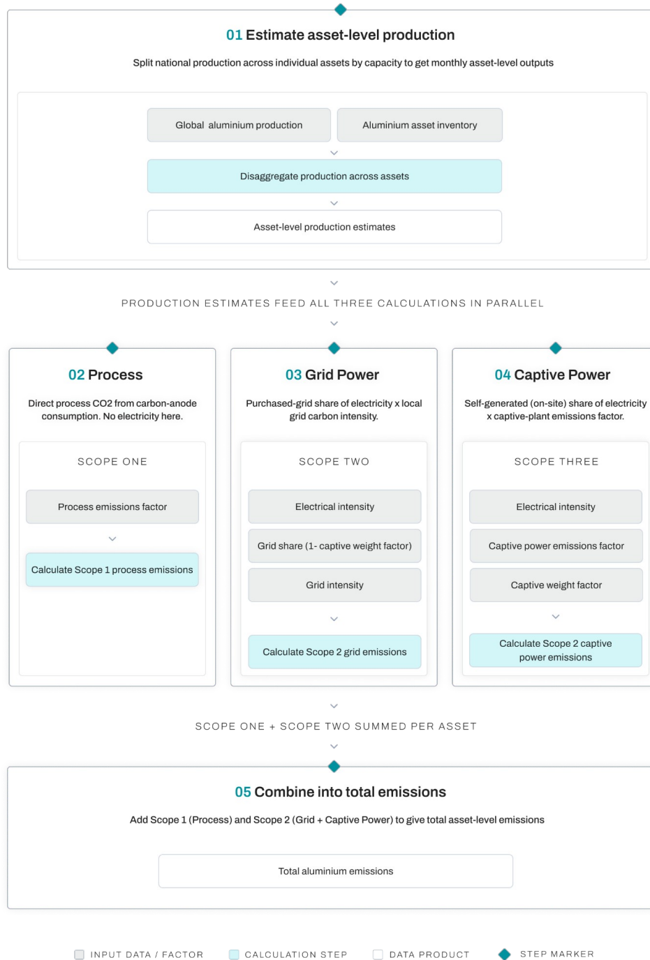
Figure 2 Flowchart of the methodology to calculate facility-level emissions for aluminum smelters and alumina refineries.
